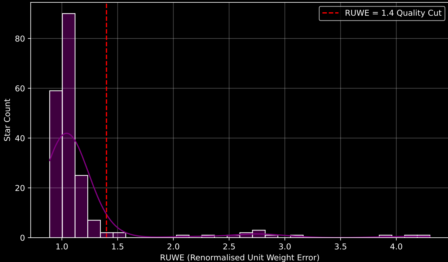
GAPOGEE DR17 Field [M35N2158] RUWE Distribution (n= 198)
