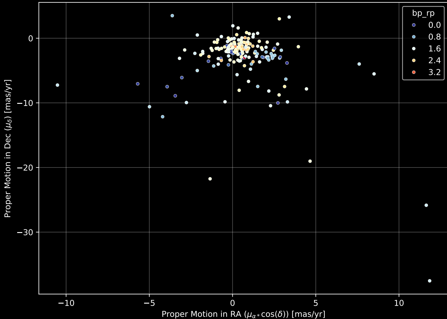
APOGEE DR17 Field: [M35N2158] Proper Motion Diagram (n= 201)
