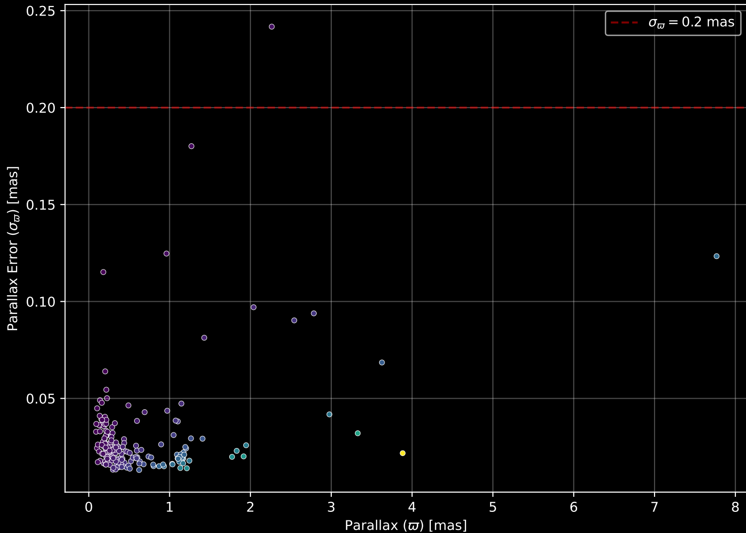
APOGEE DR17 Field: [M35N2158] Parallax Quality (n= 201)
