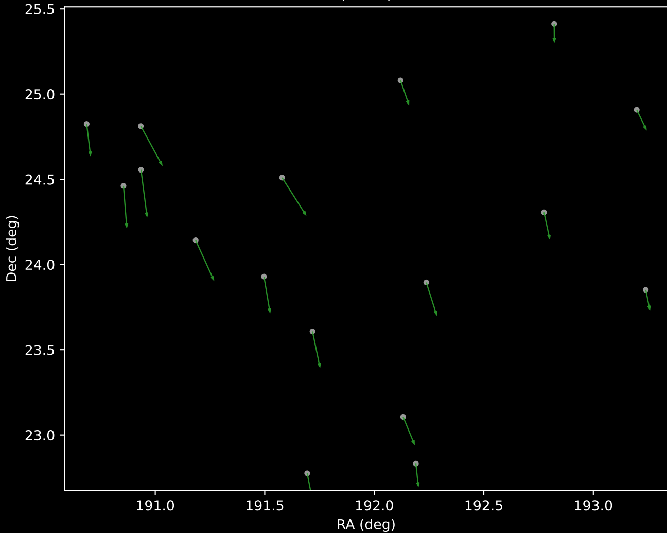
APOGEE DR17 Cluster 4 Proper Motion Vectors (n=17)
