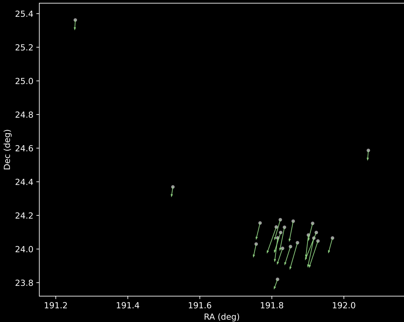
APOGEE DR17 Cluster 5 Proper Motion Vectors (n=21)
