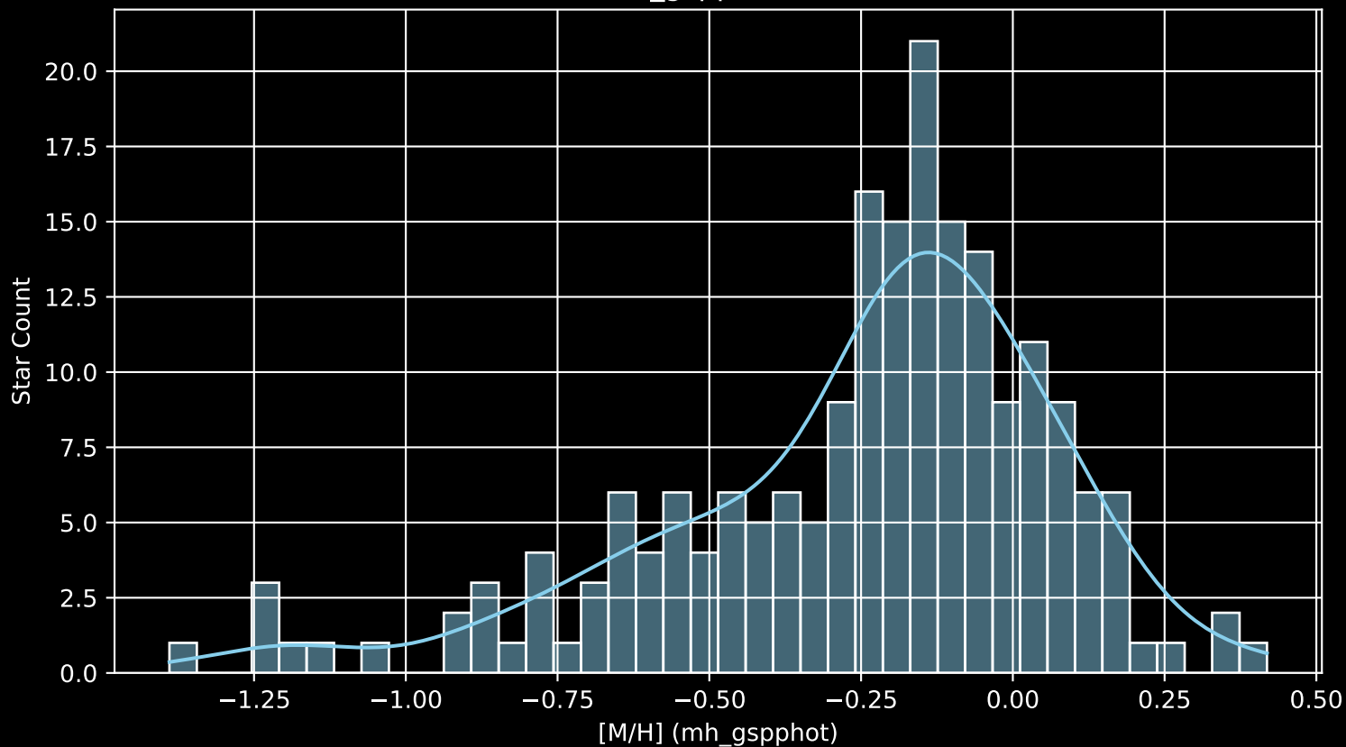
APOGEE DR17 Field: [M35N2158 [M/H] (mh_gspphot) (n= 199)
