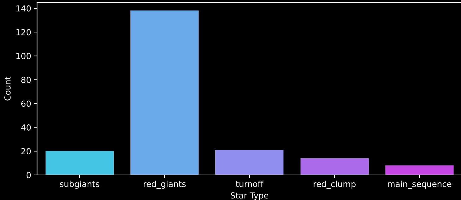
APOGEE DR17 Field: [M35N2158] Count plot of Star Type
